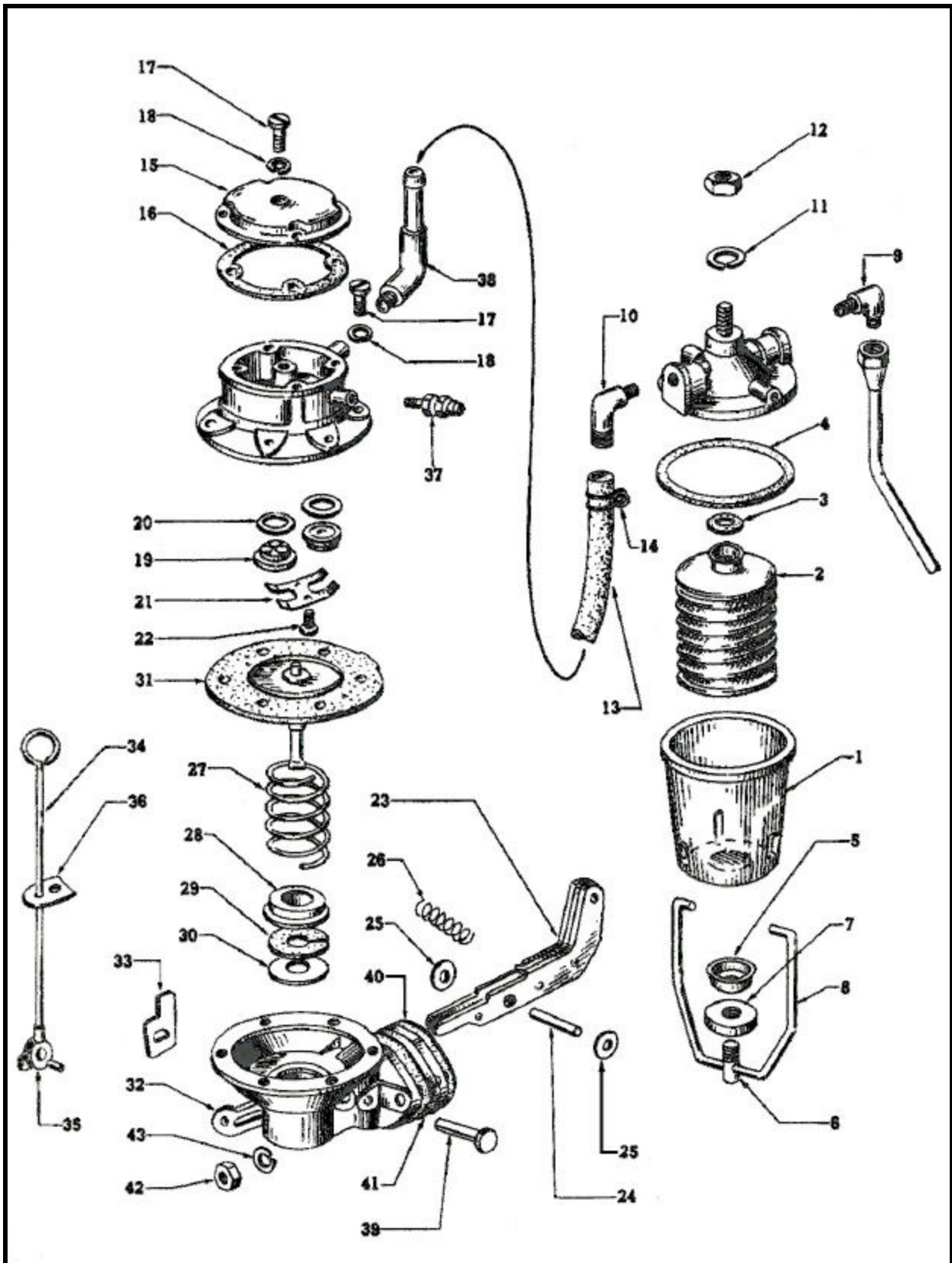
FUEL STRAINER & PUMP (SP310)
