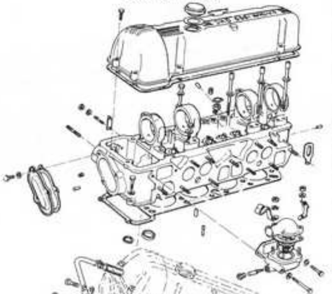
Cylinder Head
