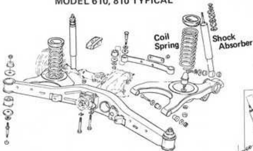
MODEL 610, 810 TYPICAL
