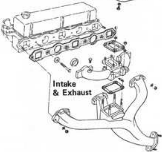
MODEL 520, J-13 Eng.
