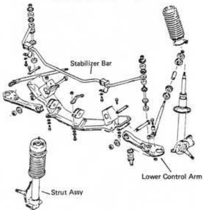
MODEL 240Z, 260Z, 280Z
