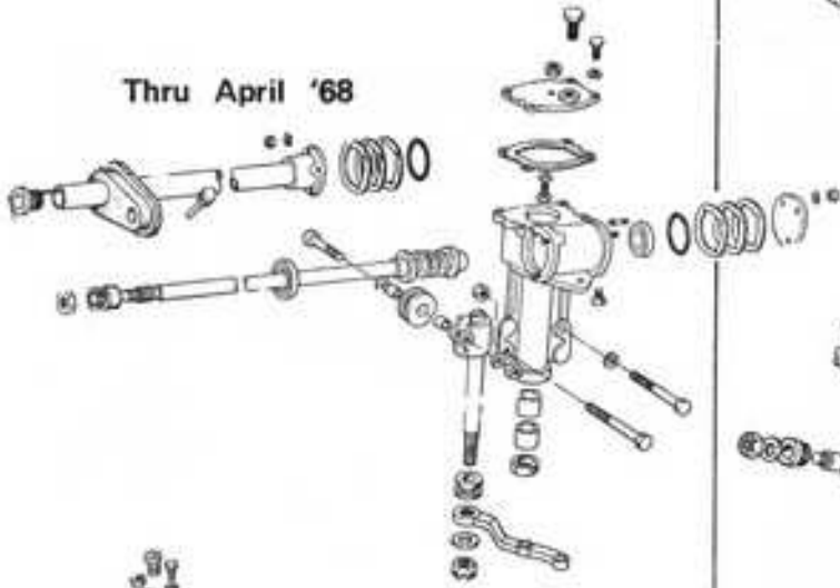
MODEL 520 & 521
