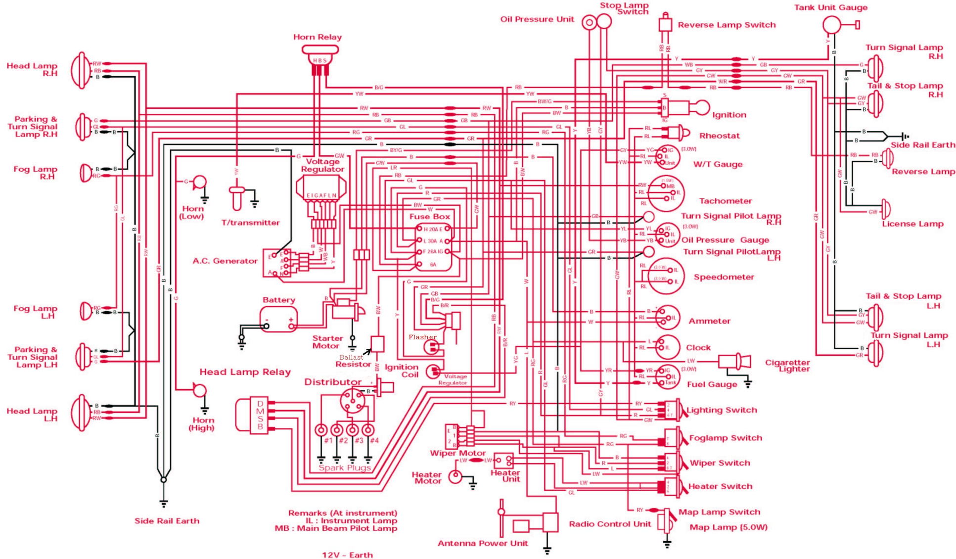
1965.5-1967 1600 SPL311 Wiring Diagram 65H67P (seven single-gauge instruments) SPL311: 00001 - 11000
